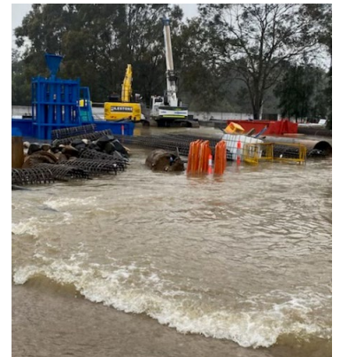
Flooding at the site compound
