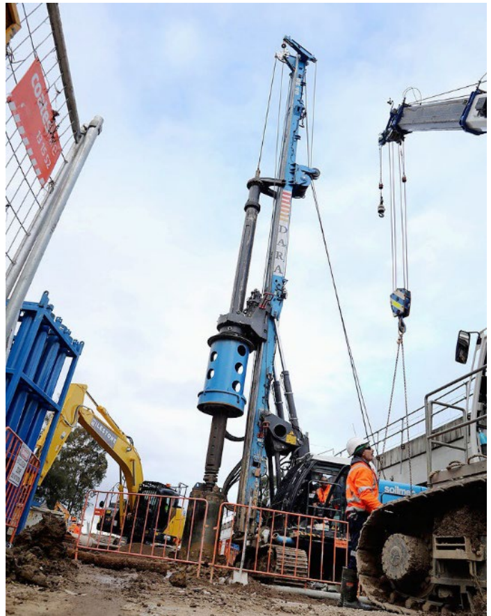
Piling activities at Sussex Street bridge
