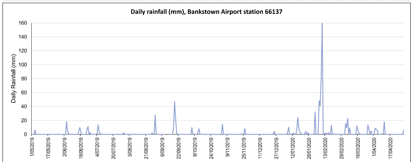
Figure 3.1 Daily rainfall at Bankstown Airport, May 2019 to April 2020
