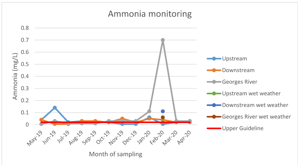
Figure 3.9 Measured ammonia (mg/L) across sites
